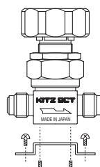
① Bottom mount
