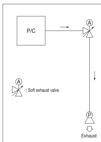
Piping layout after use of soft exhaust valve
