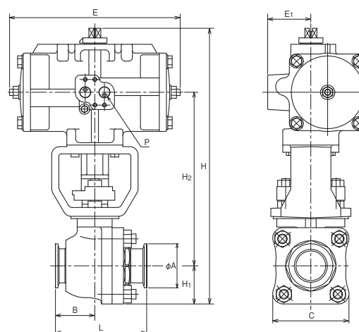
BRW series Double Acting
